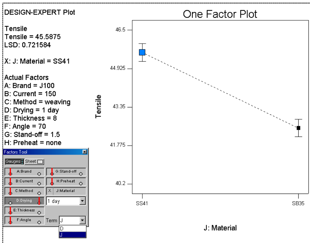
Plot of Factor J (Material) with Factor D Set at High Level and Best Point Picked
