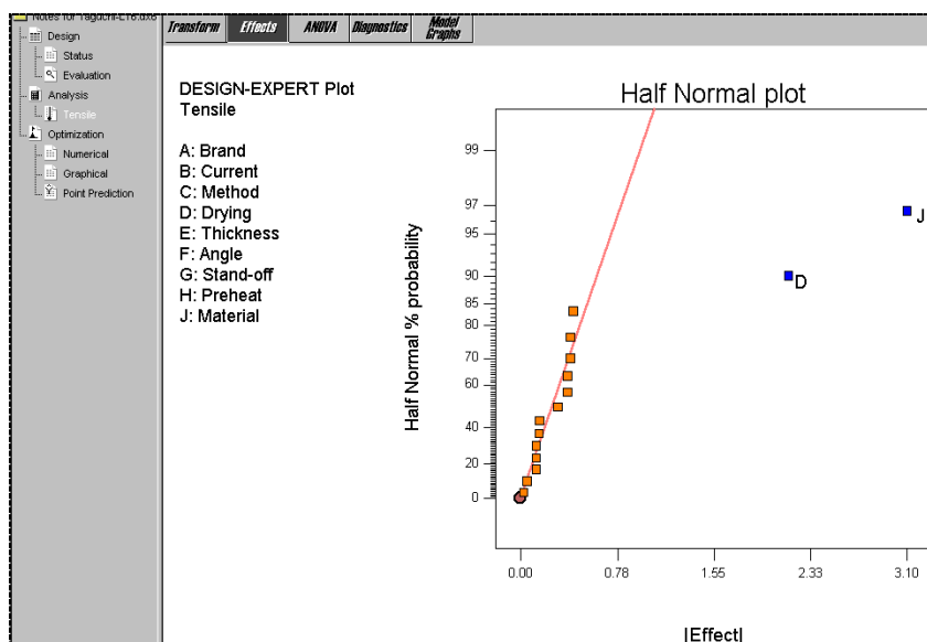
Half Normal Plot of Effects
