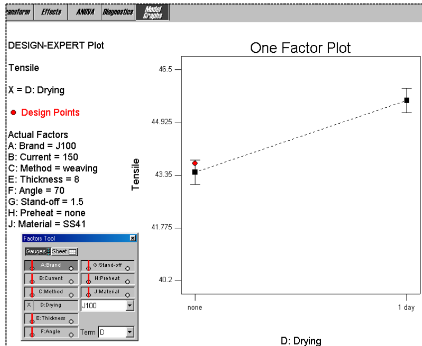
One-Factor Plot of the Effect of Factor D (Drying)
